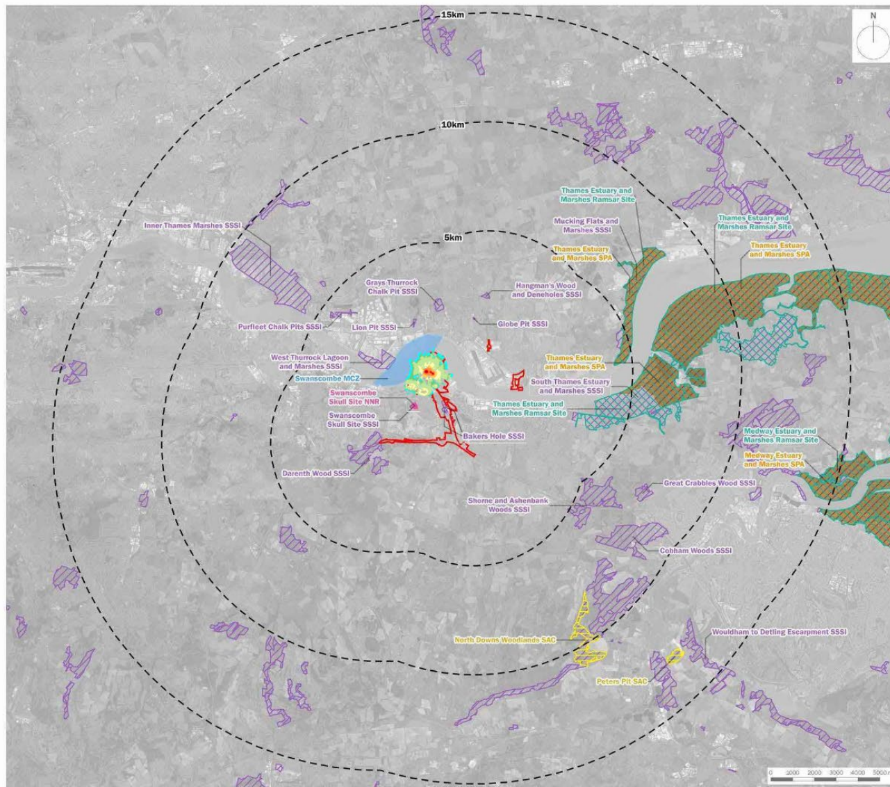
Figure 15.11: Extent of LA,max,f noise propagation from London Resort scream and mechanical ride and attraction noise to levels 5dB below the existing background noise climate (43 dB LAeq,t).
